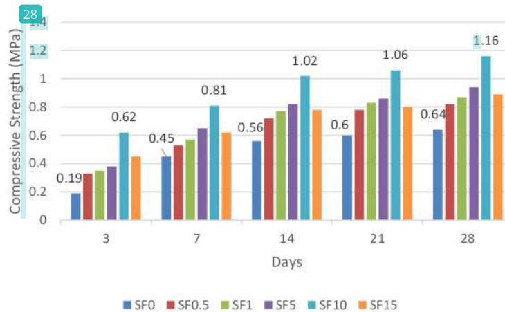
Figure. 5 Compressive strength of CLC with the added percentage of silica fume
