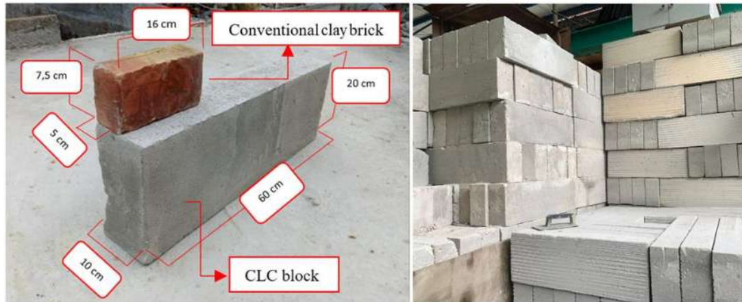
Figure 1. Cellular Lightweight Concrete blocks (a) size comparison with conventional clay brick (b) set of hardened CLC
